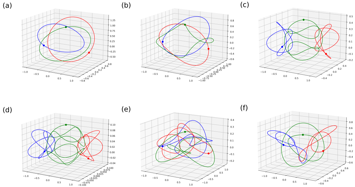
Figure 2: 3D periodic orbits of general three-body problem: (a) O_2(1.2) , (b) O_8(0.6) , (c) O_3(1.0) , (d) O_4(1.0) , (e) O_6(1.0) , (f) O_6(1.2) . Blue: Body-1; Red: Body-2; Green: Body-3. Filled circle: initial positions of the three bodies.
