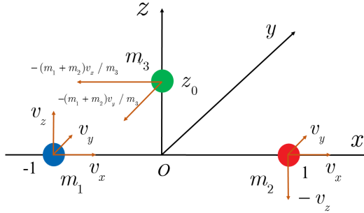
Figure 1: The initial configuration of the 3D three-body system. The initial positions of the three bodies are located at \mathbf{r}_1 = (-1, 0, 0) , \mathbf{r}_2 = (1, 0, 0) and \mathbf{r}_3 = (0, 0, z_0) with the corresponding initial velocities \mathbf{v}_1 = (v_x, v_y, v_z) , \mathbf{v}_2 = (v_x, v_y, -v_z) and \mathbf{v}_3 = (-2v_x/m_3, -2v_y/m_3, 0) .
