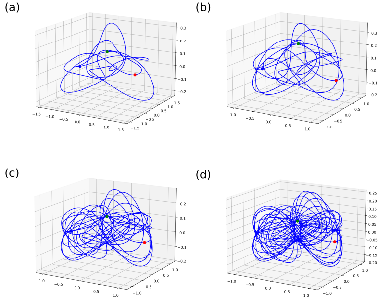
Figure 3: 3D choreographic periodic orbits of three-body problem in case of m_1 = m_2 = m_3 = 1 : (a) O_{62}(1.0) , (b) O_{64}(1.0) , (c) O_{231}(1.0) , (d) O_{524}(1.0) . Three bodies move along a single closed orbit (blue). Filled circles: the initial positions of the three bodies. Blue: Body-1; Red: Body-2; Green: Body-3.
