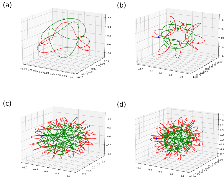
Figure 4: 3D “piano-trio orbits” of three-body problem with two bodies ( m_1 = m_2 = 1 ) moving along a single closed orbit (red) but the third ( m_3 \neq 1 ) along a distinct orbit (green): (a) O_6(0.6) , (b) O_{26}(1.1) , (c) O_{48}(0.5) , (d) O_{267}(0.9) . Filled circles: the initial positions of the three bodies. Blue: Body-1 ( m_1 = 1 ) ; Red: Body-2 ( m_2 = 1 ) ; Green: Body-3 ( m_3 \neq 1 ).
